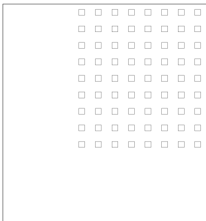
Perforation : S3 / 8.3 (Square 3 X 3mm, 8.3mm c / c)
