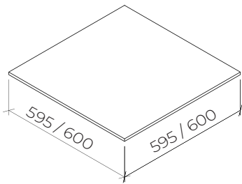
Gyptile Perforated (Lay In)
